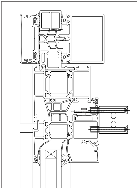
Fig. 3: Sash mounting on bottom-hung window with locking drive KLM L
