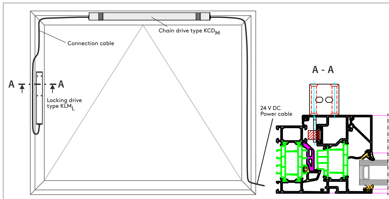
Fig. 5: Installation example on inward bottom-hung window with chain drive type KCD M and locking drive KLM L
