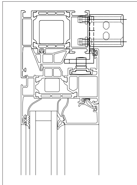
Fig. 4: Frame mounting on bottom-hung window with locking drive KLMF M
